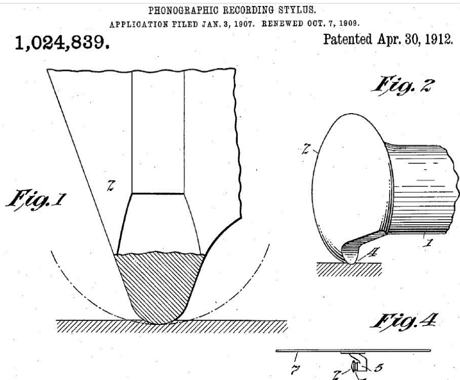
Figure (7) Recording Cutter
